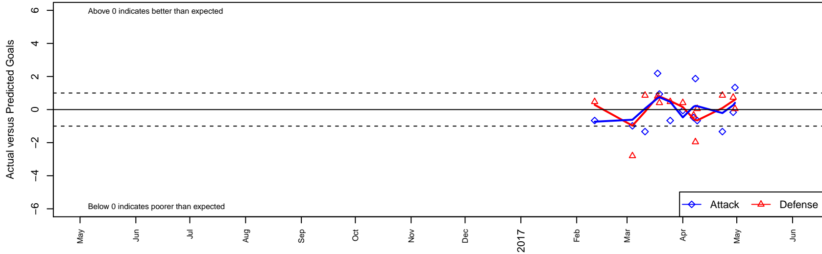
NPSA Titans Navy B05 Dots are actual minus expected GF (blue circles) and GA (red triangles). Blue line is smoothed change in attack strength. Red is smoothed change in defense strength.
